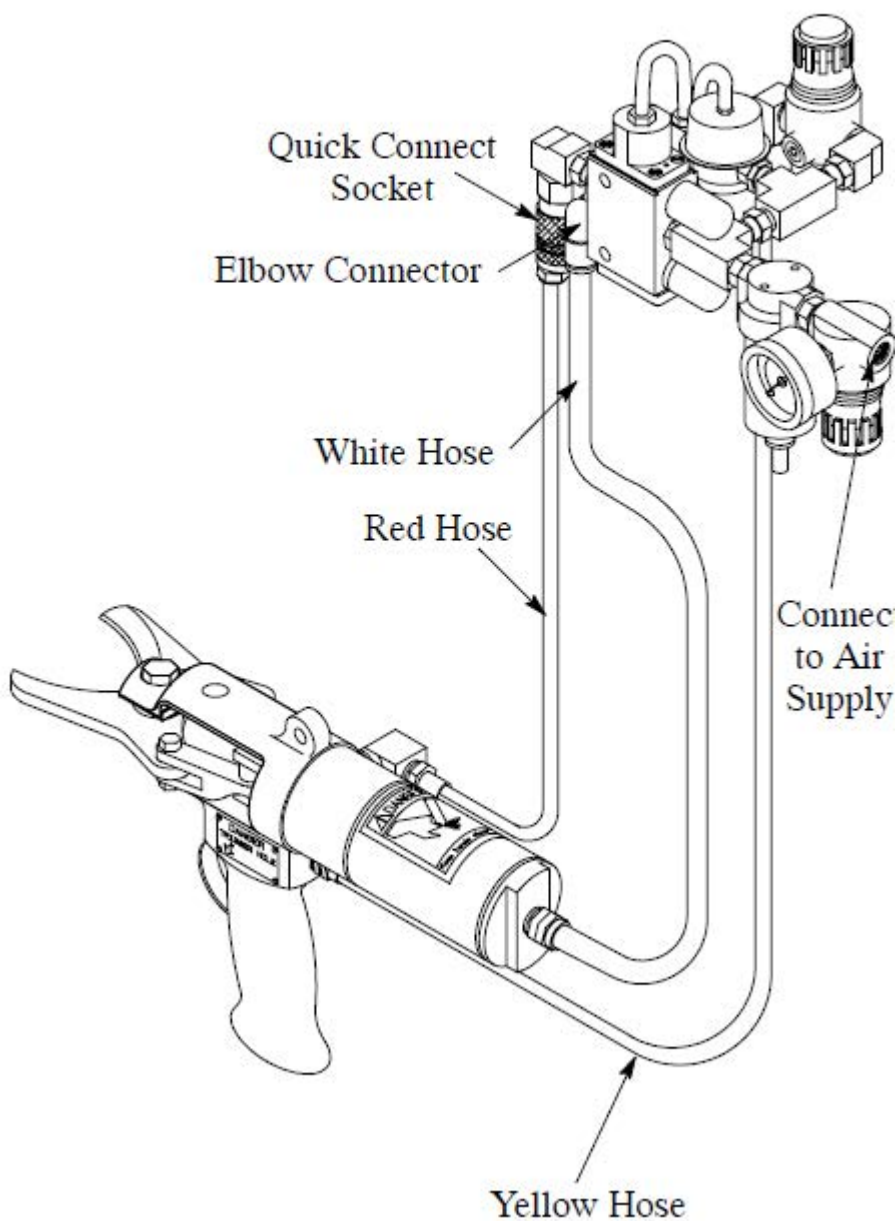
Figure 1 Hose Connection Diagram
